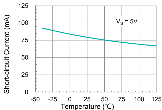
Short-circuit Current as a function of Temperature.
