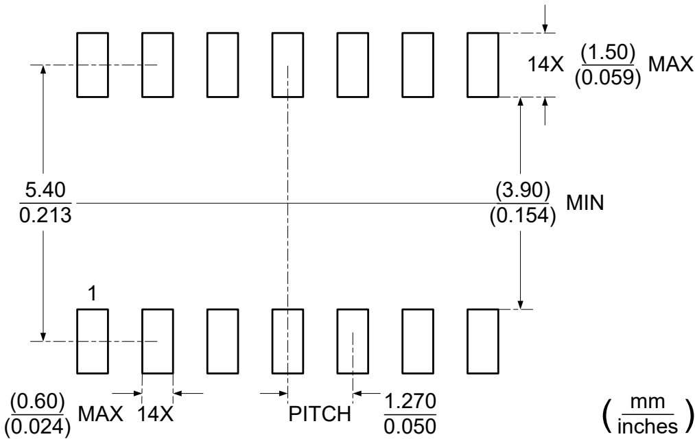
RECOMMENDED SOLDERING FOOTPRINT, SOIC-14L
