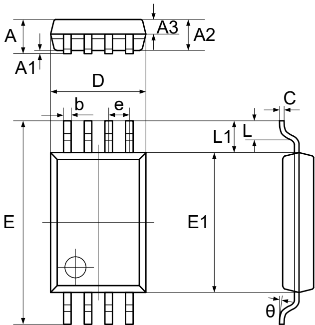
DIMENSIONS, TSSOP-8L
