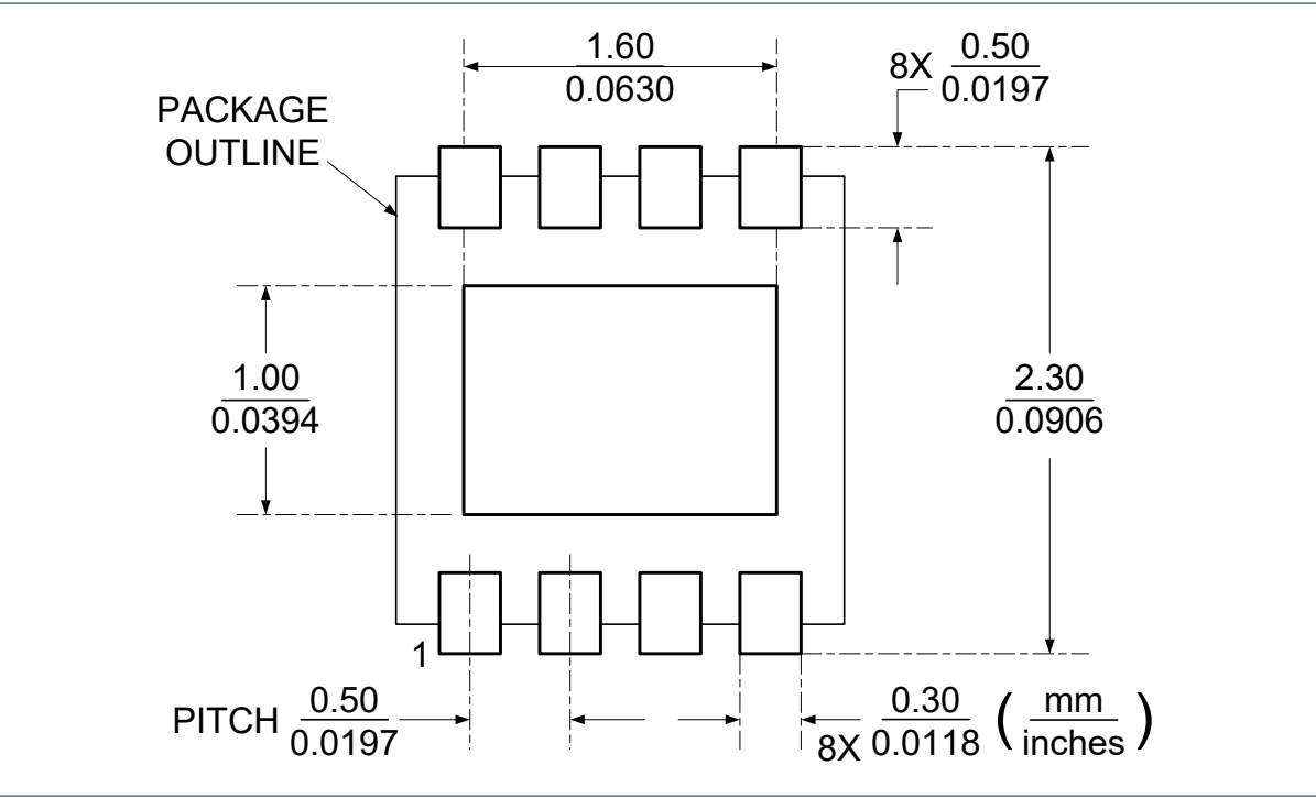
RECOMMENDED SOLDERING FOOTPRINT, DFN2x2-8L
