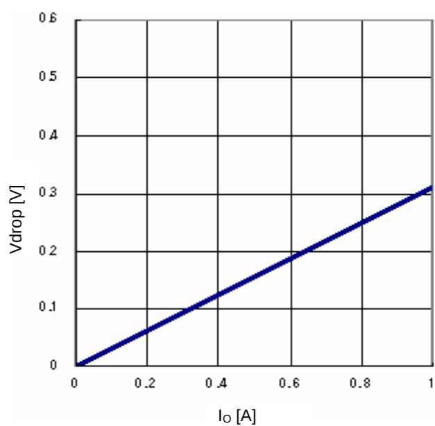
Fig.25 Minimum dropout Voltage 5 ( V_{CC}=10V , T_a=25^\circ C )
