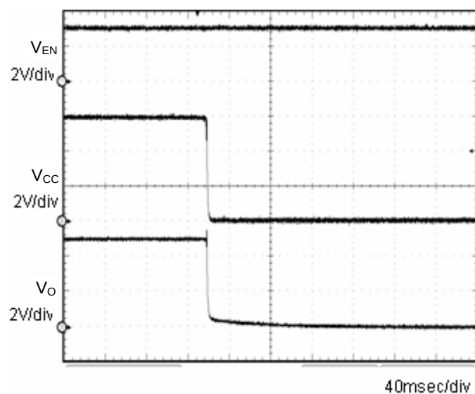
Fig.6 OFF sequence 1 C_o=1\mu\text{F}
