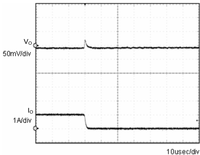
Fig.4 Transient Response (1.0→0A) C_o=1\mu\text{F}
