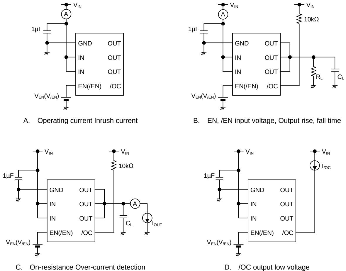
Figure 1. Measurement circuit
