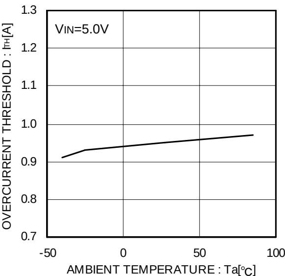
Figure 13. Over-current threshold
