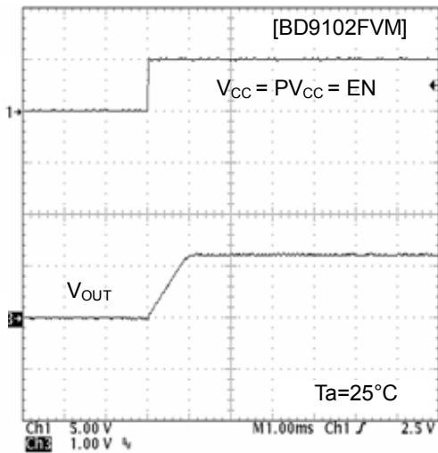
Figure 10. Soft-Start Waveform
