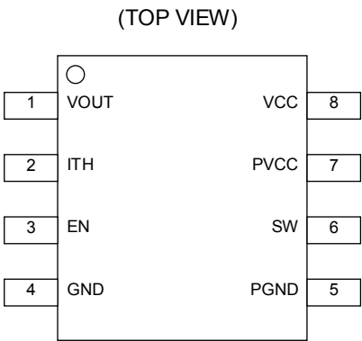
Figure 2. Pin Configuration
