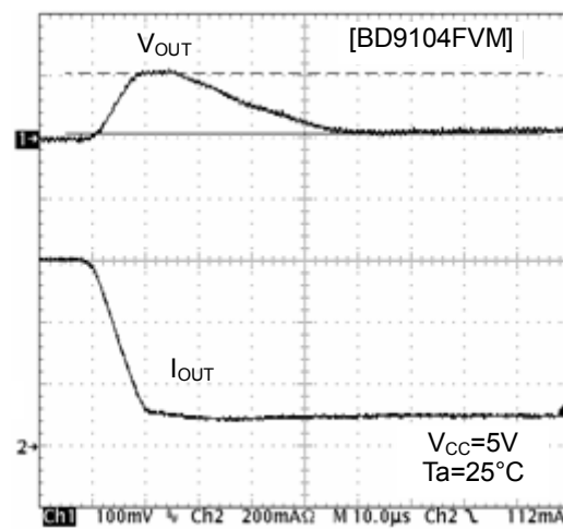
Figure 19. Transient Response ( I_O=600\text{mA} to 100\text{mA} , 10\mu s )
