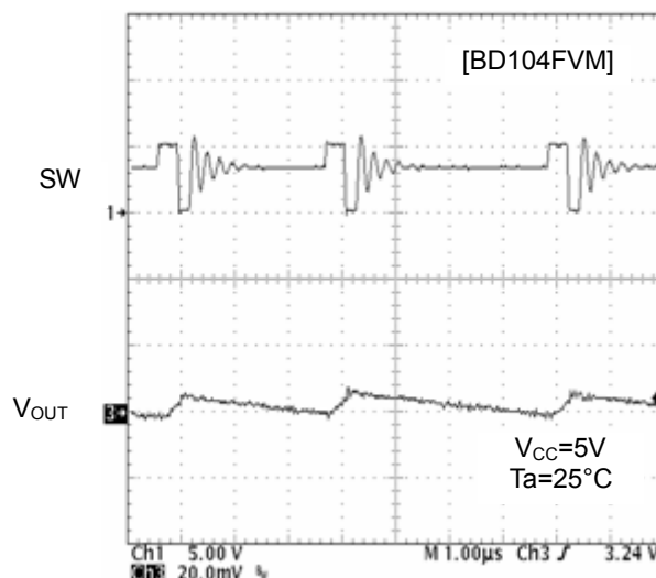
Figure 13. SW Waveform ( I_O=10\text{mA} , SLLM TM Control)
