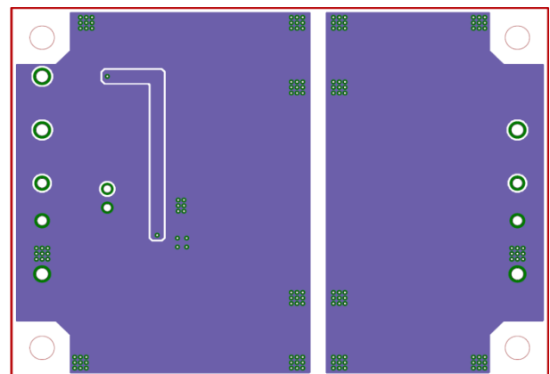
Figure 10. Bottom Side Layer Layout (Top View)
