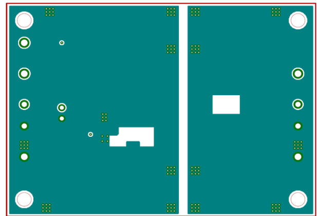
Figure 8. Middle Layer1 Layout (Top View)
