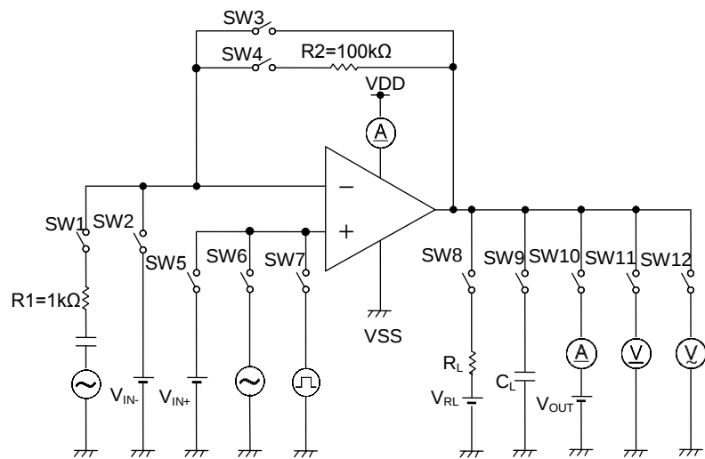
Figure 31. Test Circuit 2
