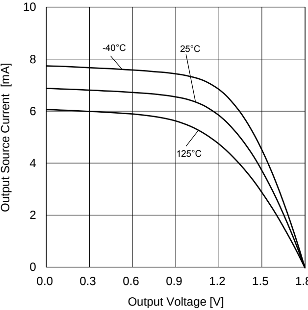
Figure 9. Output Source Current vs Output Voltage ( V_{DD}=1.8\text{ V} )
