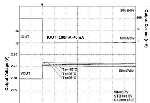
Fig 170. Load Response
