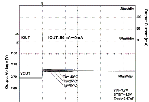
Fig 168. Load Response
