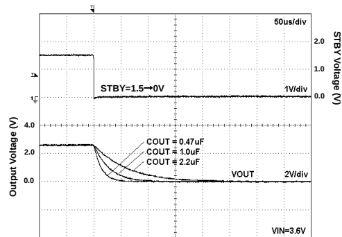
Fig 153. Discharge Time
