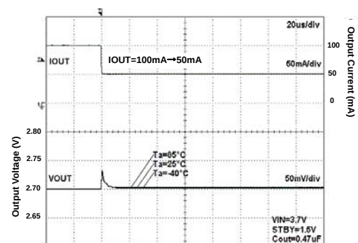
Fig 174. Load Response
