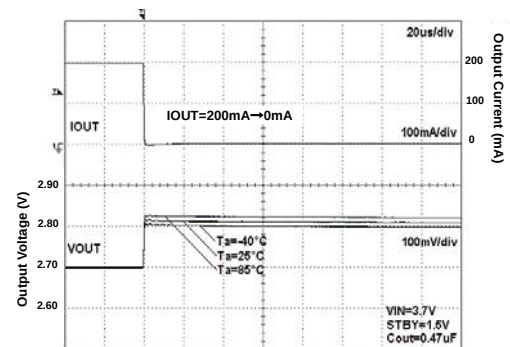
Fig 172. Load Response
