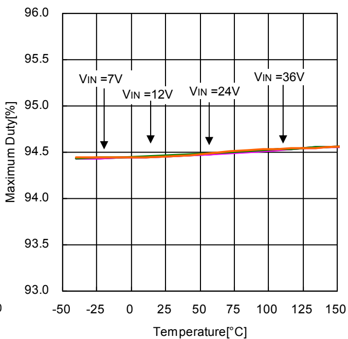
Figure 9. Maximum Duty vs Junction Temperature
