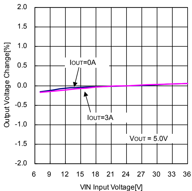
Figure 30. VOUT Line Regulation
