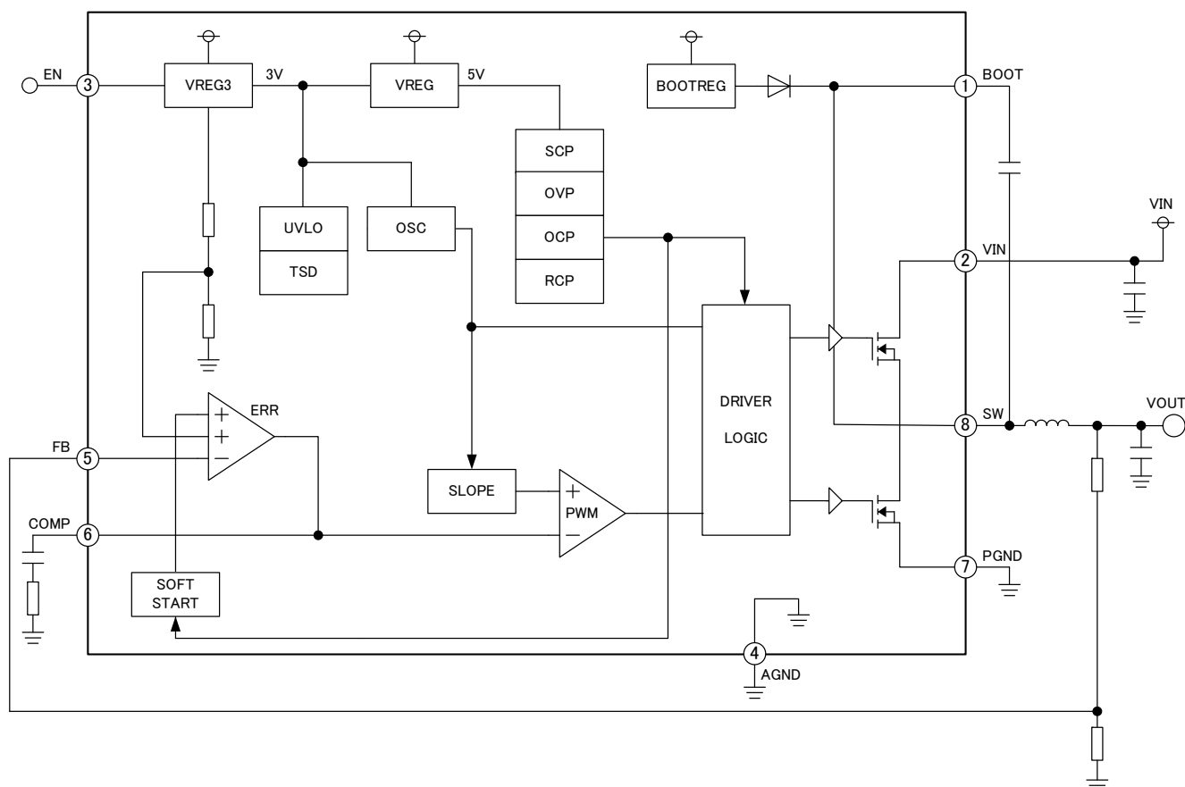
Figure 3. Block diagram
