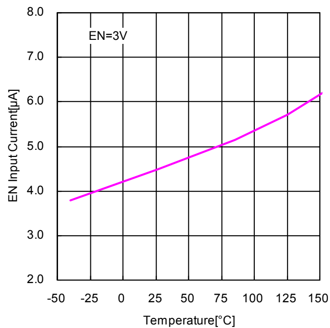
Figure 15. EN Input Current vs Junction Temperature
