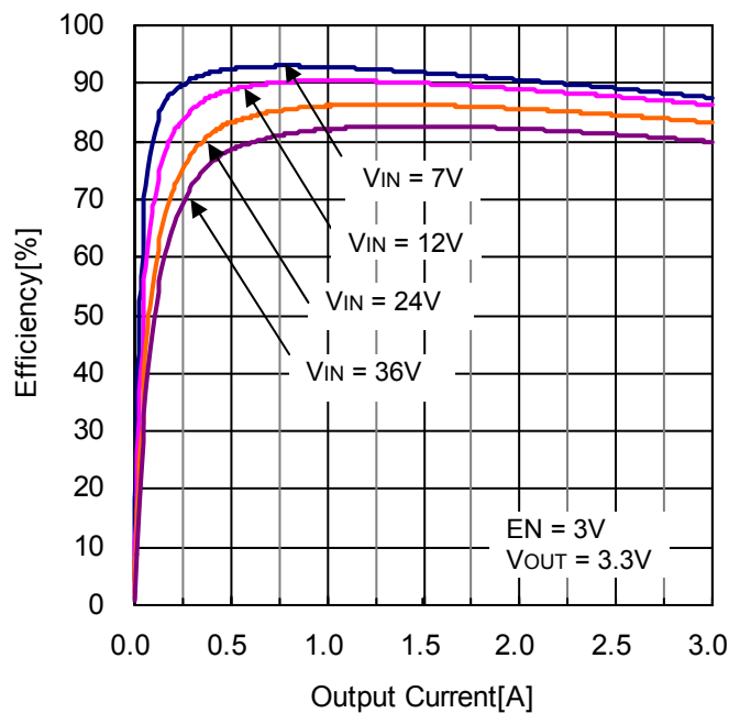
Figure 17. Efficiency vs Output Current ( V_{OUT} = 3.3V , L = 10\mu H )
