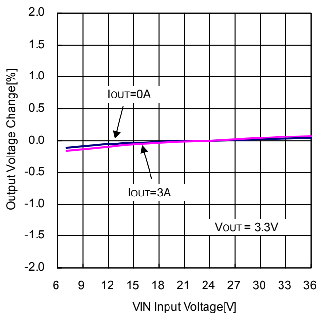
Figure 29. VOUT Line Regulation
