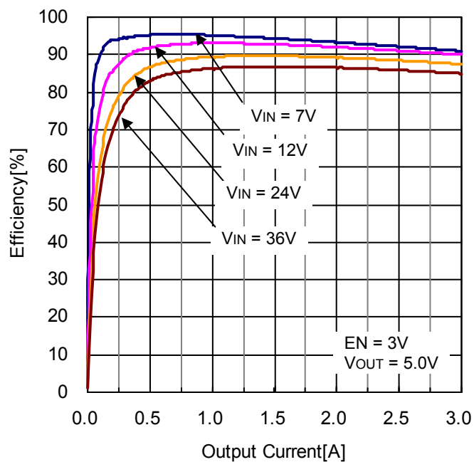
Figure 18. Efficiency vs Output Current ( V_{OUT} = 5.0V , L = 10\mu H )
