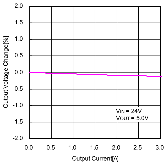
Figure 32. VOUT Load Regulation ( V_{OUT} = 5.0V )
