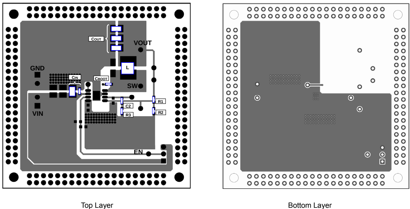
Figure 47. Example of Sample Board Layout Pattern
