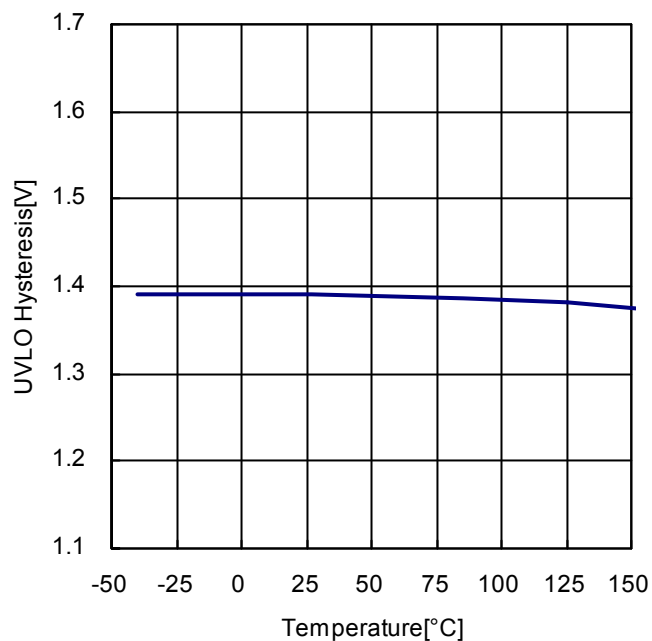
Figure 13. UVLO Hysteresis vs Junction Temperature
