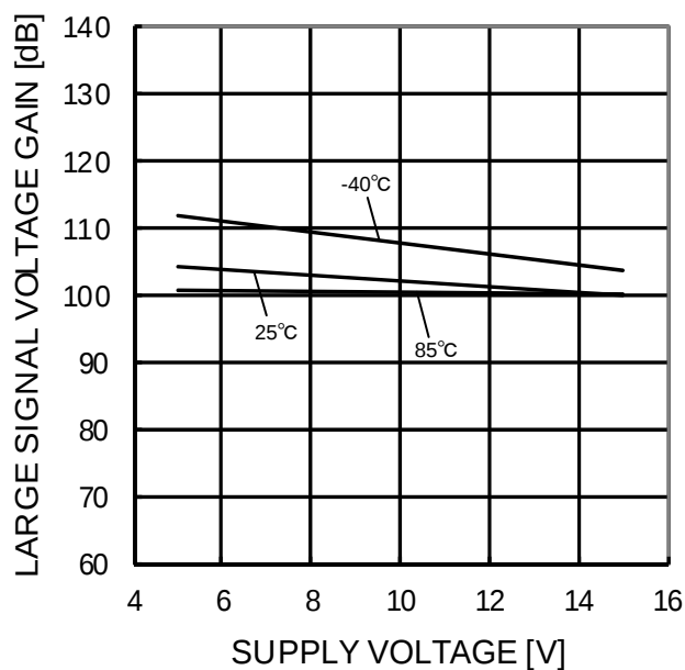
Figure 45. Large Signal Voltage Gain - Supply Voltage (R L =2kΩ)
