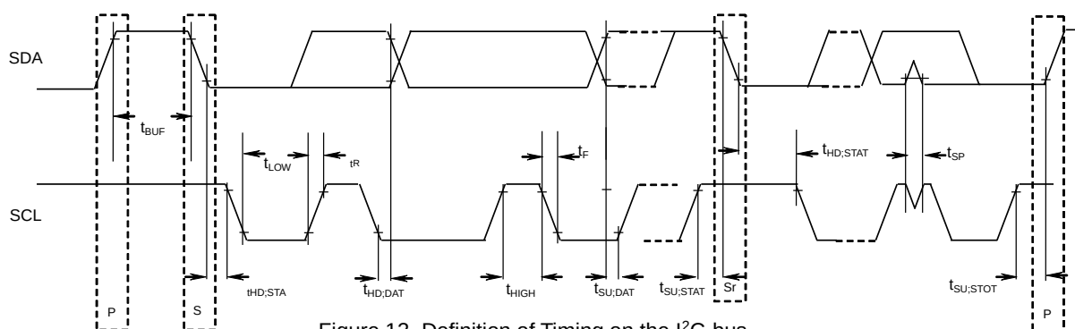
Figure 13. Definition of Timing on the I 2 C-bus
