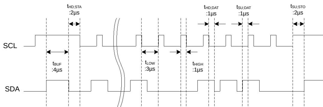
Figure 14. A Command Timing Example in the I 2 C Data Transmission
