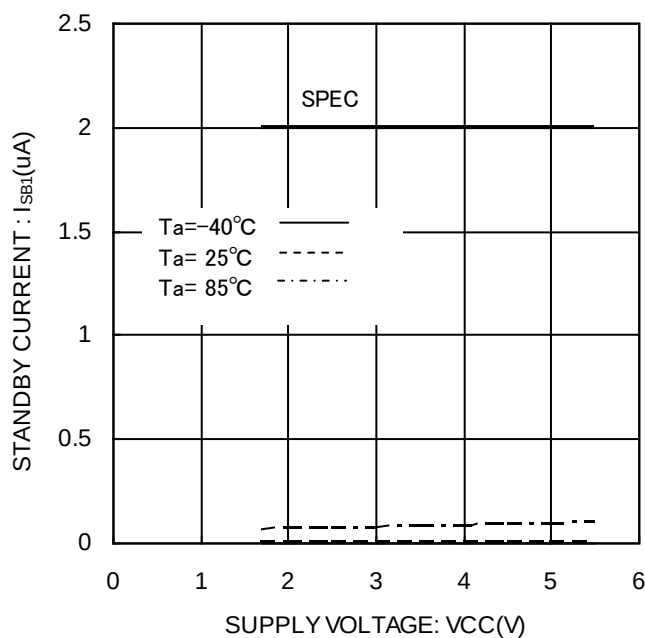
Figure 19. Standby current I_{SBI}(\text{CS}=0\text{V}, \text{ORG}=\text{VCC or OPEN})
