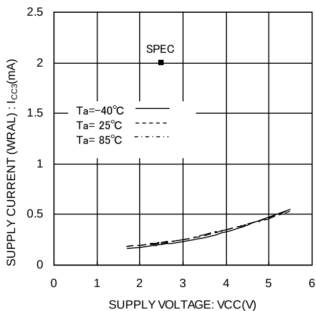
Figure 17. Supply current (WRAL) I_{CC3} [\text{WRAL}, f_{SK}=1\text{MHz}]
