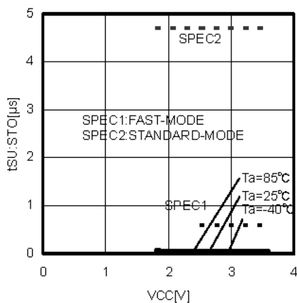
Figure 22. Stop Condition Setup Time t_{SU:STO}
