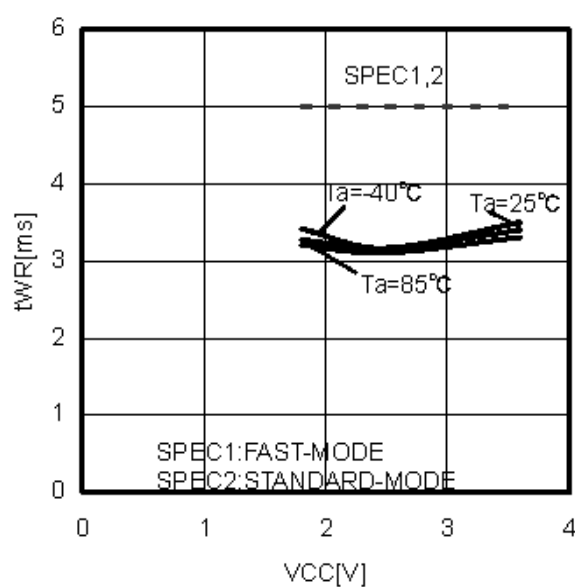
Figure 24. Write Cycle Time t_{WR}
