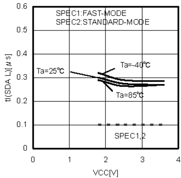
Figure 28. Noise Spike Width tI (SDA L)
