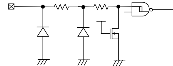
Figure 51. Input Pin Circuit
