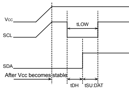
Figure 53. SCL='H' and SDA='L'
