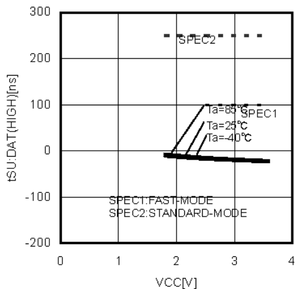
Figure 18. Input Data Setup Time t_{SU:DAT(HIGH)}
