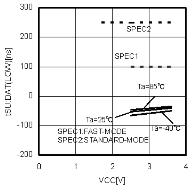
Figure 19. Input Data Setup Time t_{SU:DAT(LOW)}
