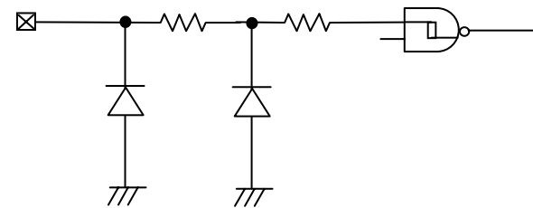
Figure 50. Input Pin Circuit
