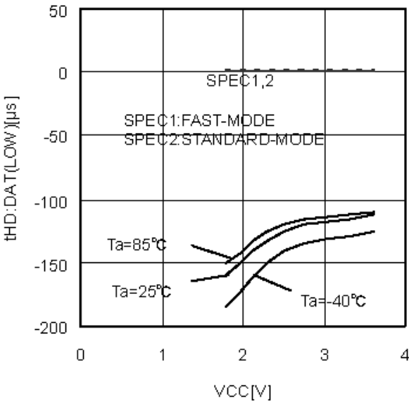
Figure 17. Data Hold Time tHD:DAT(LOW)
