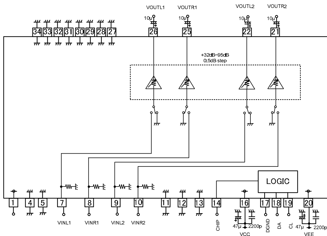
Figure 1. Application Circuit
