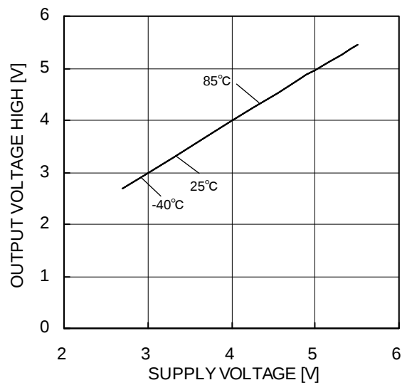
Figure 53. Maximum Output Voltage(High) – Supply Voltage ( R_L=2\text{ k}\Omega )
