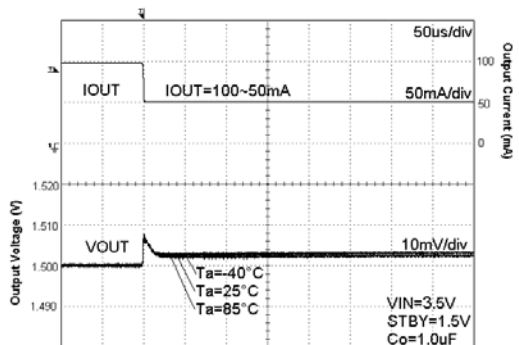
Fig. 23 Load Response
