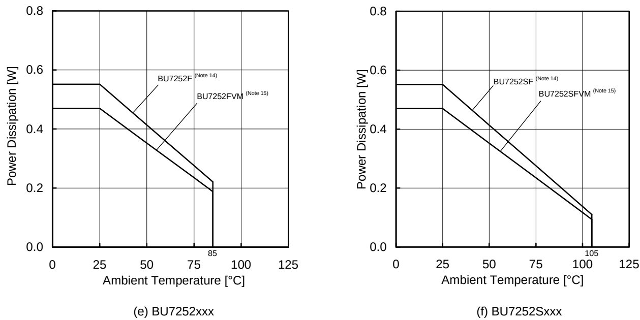
Figure 48. Thermal Resistance and Derating Curve
