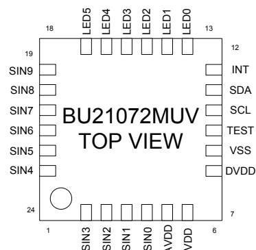
Figure 2. Pin configuration (BU21072MUV)
