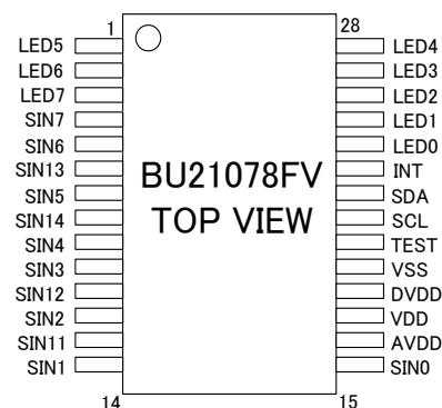
Figure 4. Pin configuration (BU21078FV)
