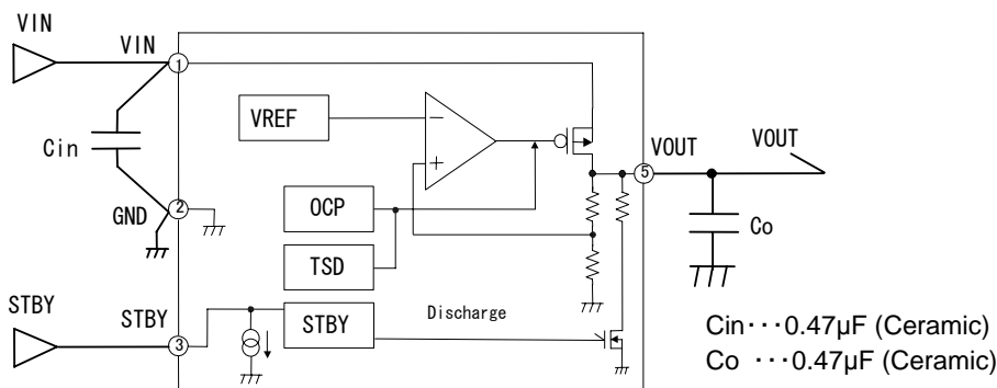
Fig. 2 Block Diagrams
