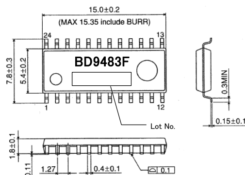
Figure 4-1. SOP-24
