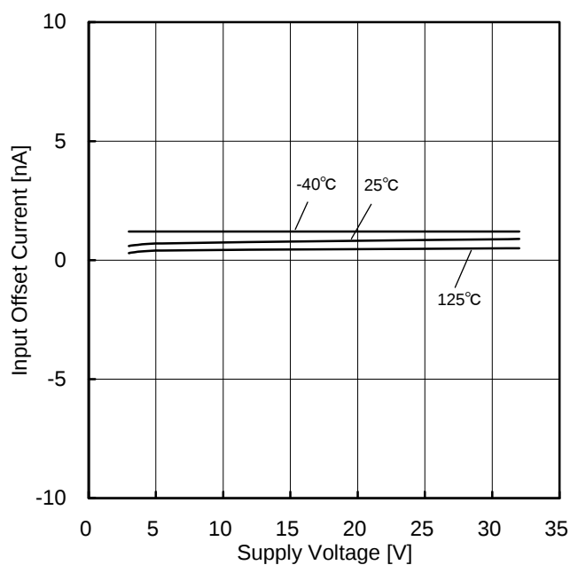
Figure 19. Input Offset Current vs Supply Voltage (VICM=0V, EK=-1.4V)
