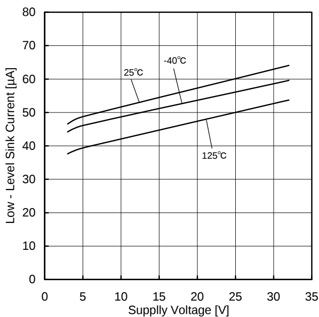
Figure 11. Low Level Sink Current vs Supply Voltage (OUT=0.2V)
