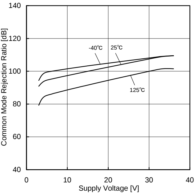
Figure 47. Common Mode Rejection Ratio vs Supply Voltage
