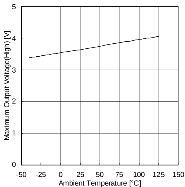
Figure 30. Maximum Output Voltage(High) vs Ambient Temperature (VCC=5V, R_L=2k\Omega )
