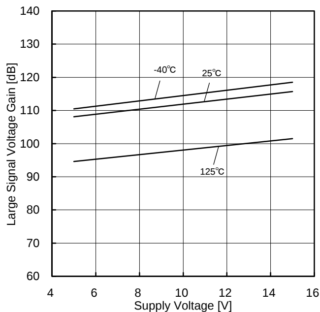
Figure 45. Large Signal Voltage Gain vs Supply Voltage ( R_L=2k\Omega )
