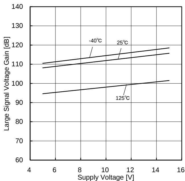
Figure 21. Large Signal Voltage Gain vs Supply Voltage (RL=2kΩ)
