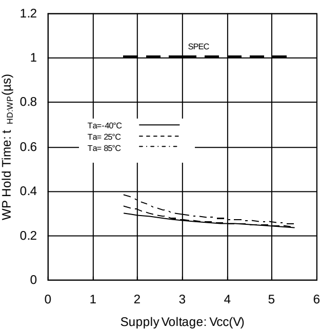
Figure 31. WP Hold Time vs Supply Voltage
