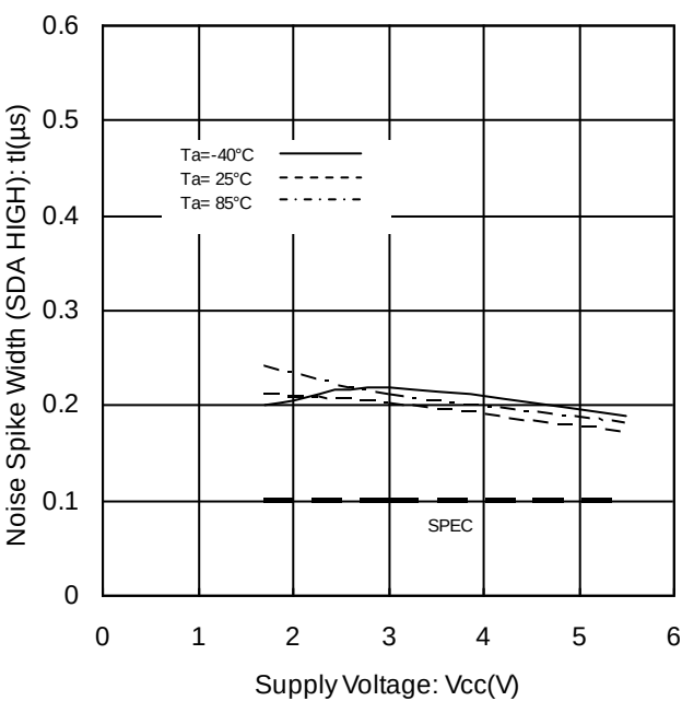
Figure 29. Noise Spike Width vs Supply Voltage (SDA HIGH)
