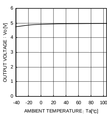
Fig.20 Output Voltage Temperature Characteristics
