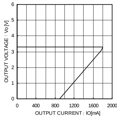
Fig.5 Load Regulation
