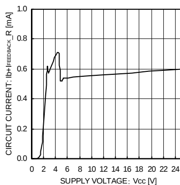
Fig.13 Circuit Current
