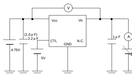
Measurement Circuit of Fig.6 and Fig.18
