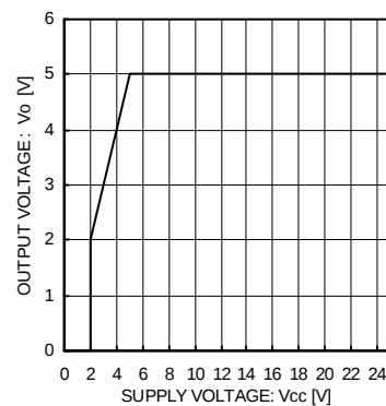
Fig.15 Line Regulation ( I_o=0\text{mA} )
