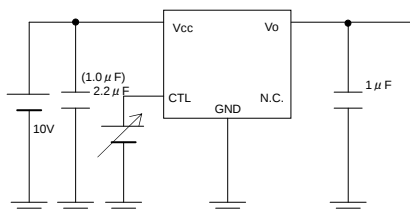
Measurement Circuit of Fig.11 and Fig.23
