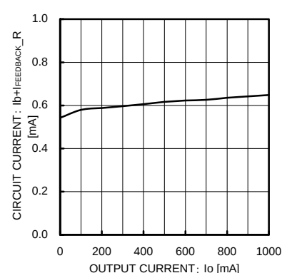
Fig.21 Circuit Current ( I_o=0\text{mA} \rightarrow 1000\text{mA} )
