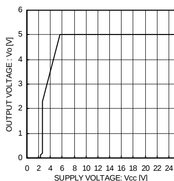
Fig.16 Line Regulation ( I_o=500\text{mA} )
