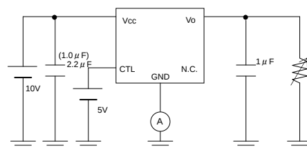
Measurement Circuit of Fig.9 and Fig.21
