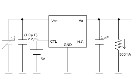
Measurement Circuit of Fig.4 and Fig.16
