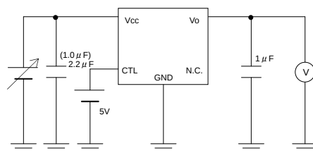
Measurement Circuit of Fig.3 and Fig.15
