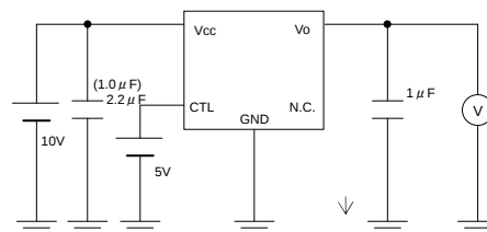
Measurement Circuit of Fig.12 and Fig.24
