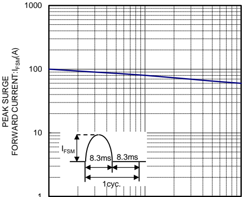
I_FSM-CYCLE CHARACTERISTICS
