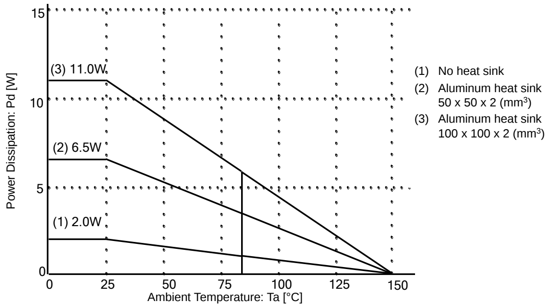
Figure 17. Power Dissipation
