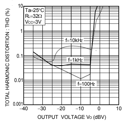
Fig. 6 Total harmonic distortion vs. output voltage (2)
