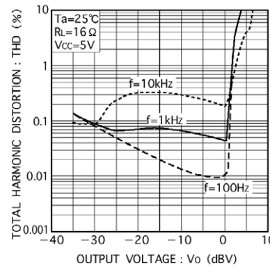
Fig. 8 Total harmonic distortion vs. output voltage (4)
