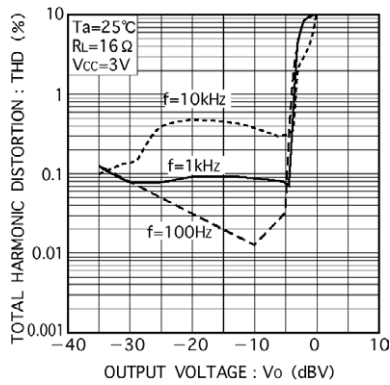
Fig. 7 Total harmonic distortion vs. output voltage (3)
