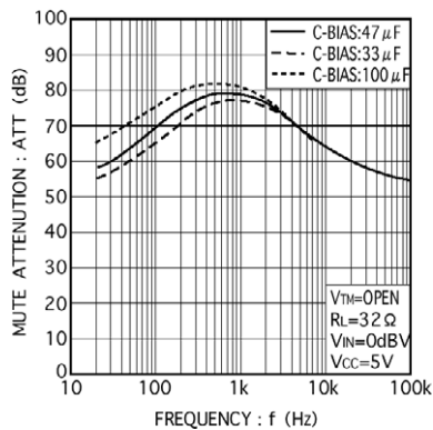
Fig. 10 MUTE attenuation vs. frequency
