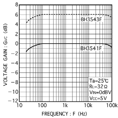
Fig. 4 Voltage gain vs. frequency
