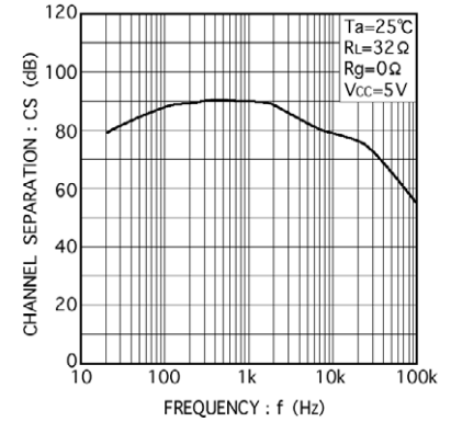
Fig. 9 Channel separation vs. frequency
