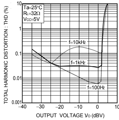
Fig. 5 Total harmonic distortion vs. output voltage (1)
