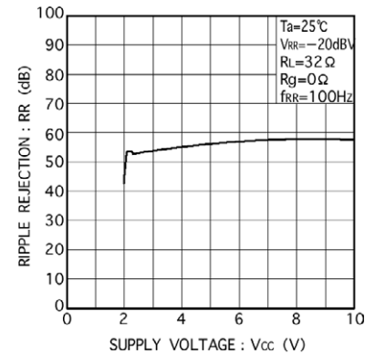
Fig. 12 Ripple rejection vs. power supply voltage
