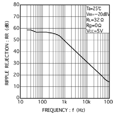
Fig. 11 Ripple rejection vs. frequency
