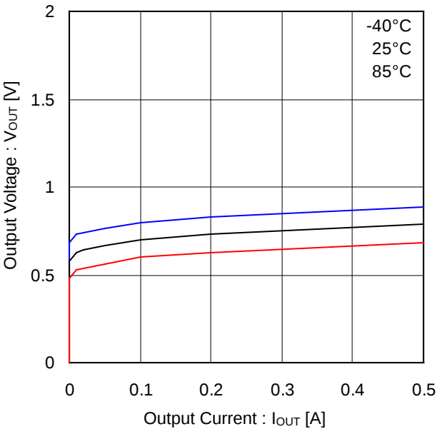
Figure 34. Output Voltage vs Output Current (Low Side Body Diode, BD6230)
