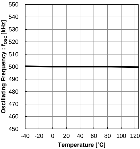
Figure 22. Oscillating Frequency vs Temperature
