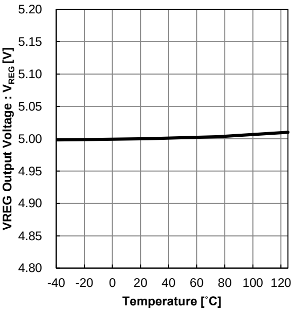
Figure 20. VREG Output Voltage vs Temperature
