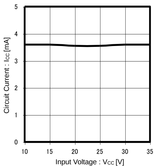
Figure 8. Circuit Current vs Input Voltage (No Load)
