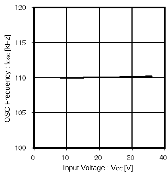
Figure 10. OSC Frequency vs Input Voltage
