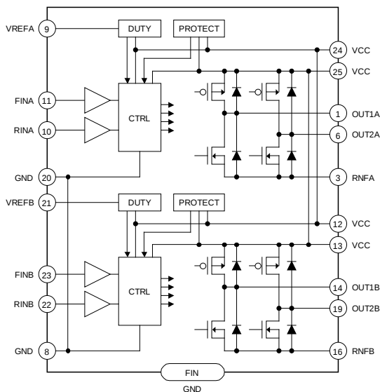
Figure 7. BD6225FP / BD6226FP
