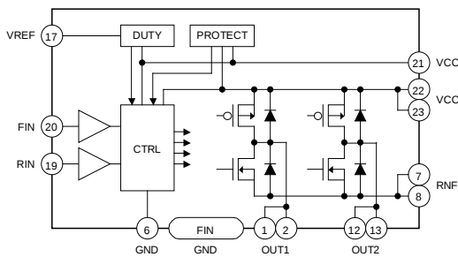
Figure 5. BD6222FP
