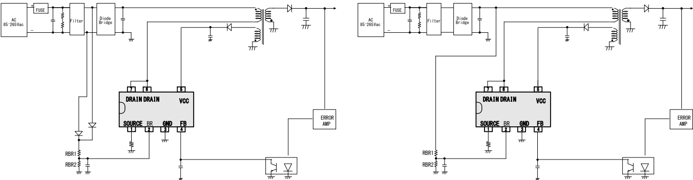
Figure 16(a). AC voltage monitor setting Figure 16(b). DC voltage monitors setting
