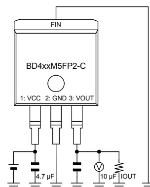
Measurement Setup for Figure 9, 27
