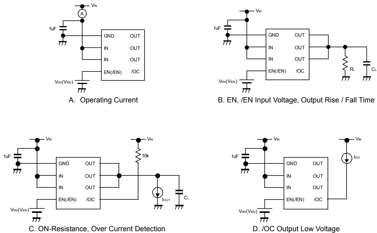
Figure 1. Measurement Circuit
