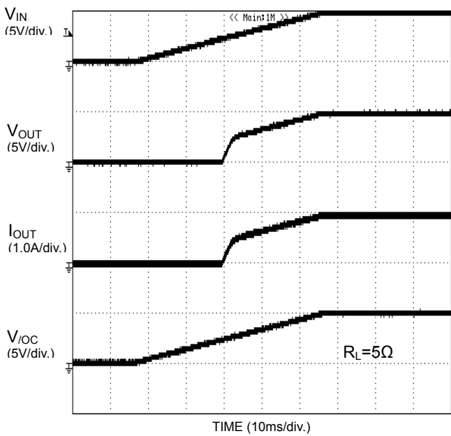
Figure 36. UVLO Response Increasing V_{IN} (BD2061AFJ)
