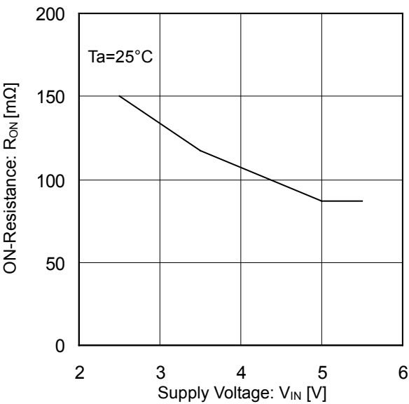
Figure 12. ON-Resistance vs Supply Voltage
