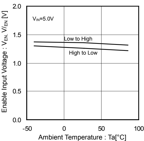
Figure 9. EN, /EN Input Voltage vs Ambient Temperature
