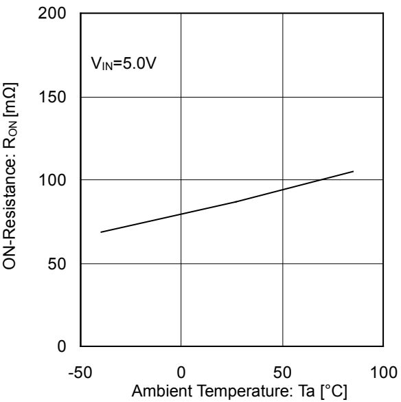
Figure 13. ON-Resistance vs Ambient Temperature
