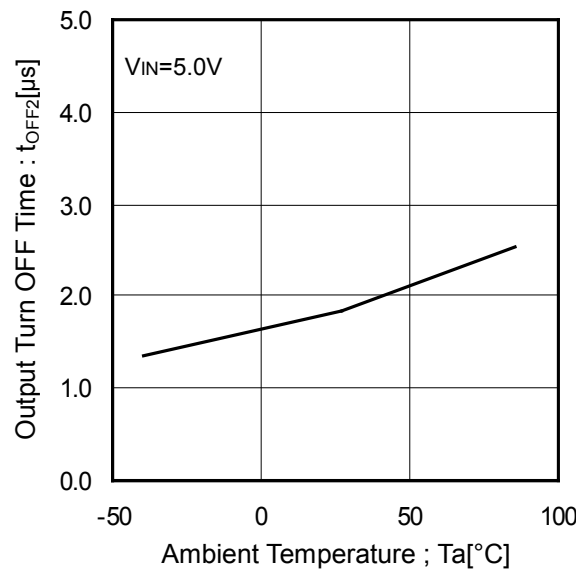
Figure 25. Output Turn OFF Time vs Ambient Temperature
