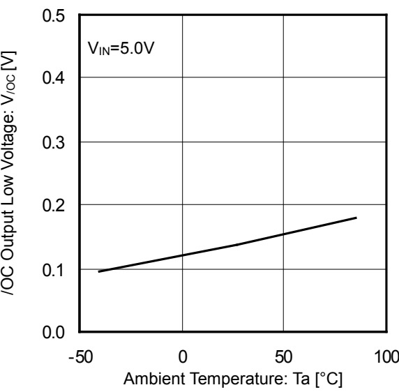
Figure 11. /OC Output Low Voltage vs Ambient Temperature
