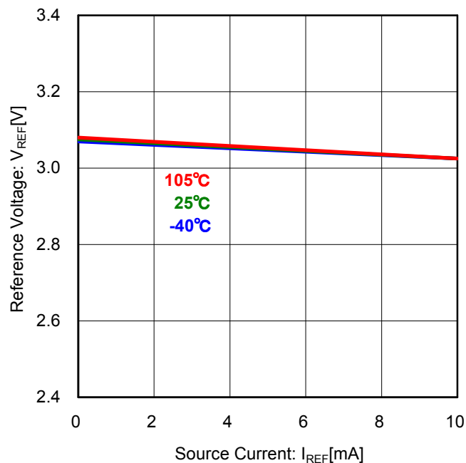
Figure 6. Reference Voltage vs Source Current ( V_{CC}=12V )
