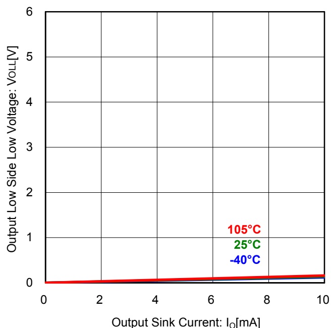
Figure 12. Low Side Output Low Voltage vs Sink Current ( V_{CC}=12V )
