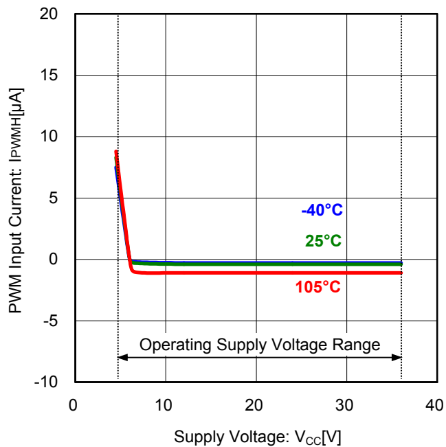
Figure 4. PWM Input Current vs Supply Voltage ( V_{PWM}=5V )
