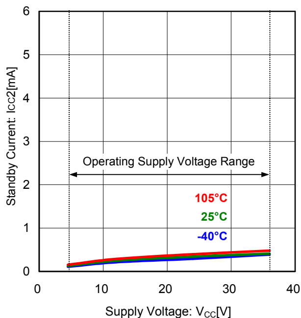
Figure 2. Standby Current vs Supply Voltage
