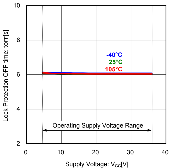
Figure 16. Lock Protection OFF Time vs Supply Voltage
