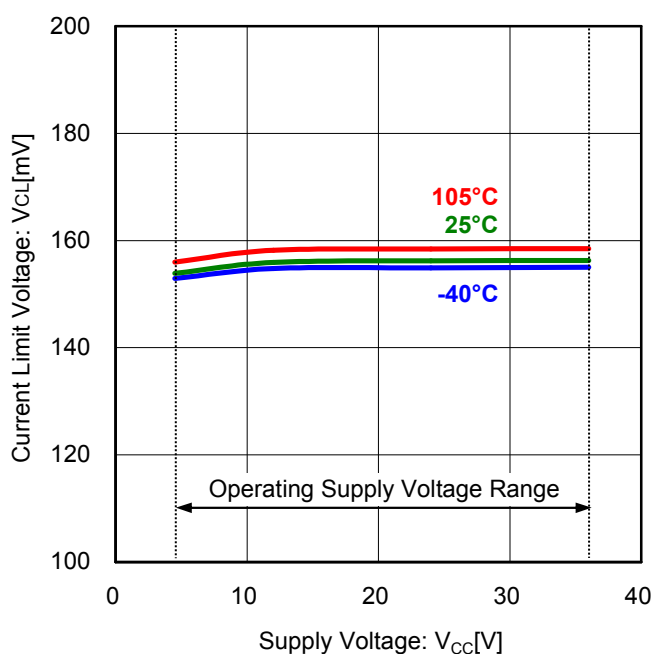
Figure 8. Current Limit Voltage vs Supply Voltage
