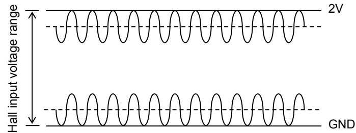
Figure 42. Hall Input Voltage Range
