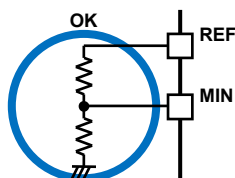
Resistor Divider
