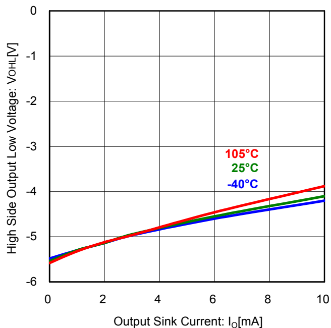
Figure 10. High Side Output Low Voltage vs Sink Current ( V_{CC}=12V , differential voltage to V_{CC} )
