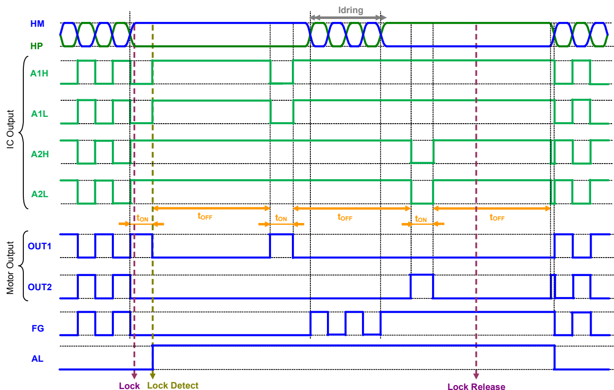
Figure 41. Lock Protection Timing Chart
