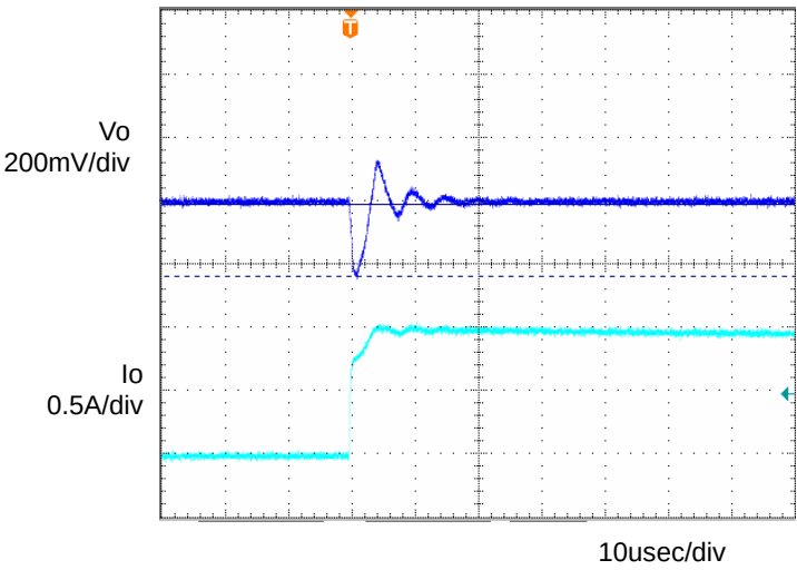
Fig.4 Transient Response (1.0→0A) Co=1μF, Ta=25°C
