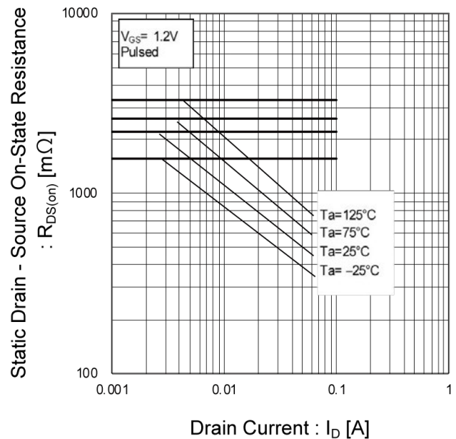
Fig.17 Static Drain - Source On - State Resistance vs. Drain Current (V)
