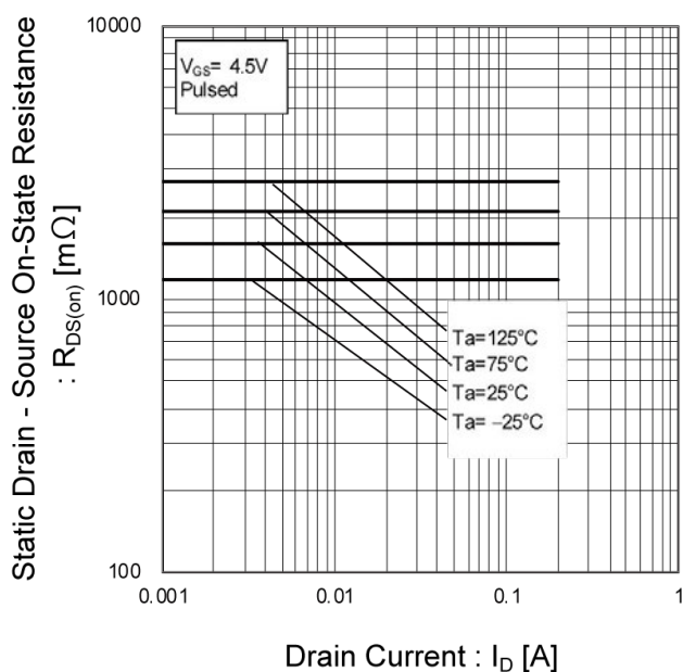
Fig.14 Static Drain - Source On - State Resistance vs. Drain Current (II)
