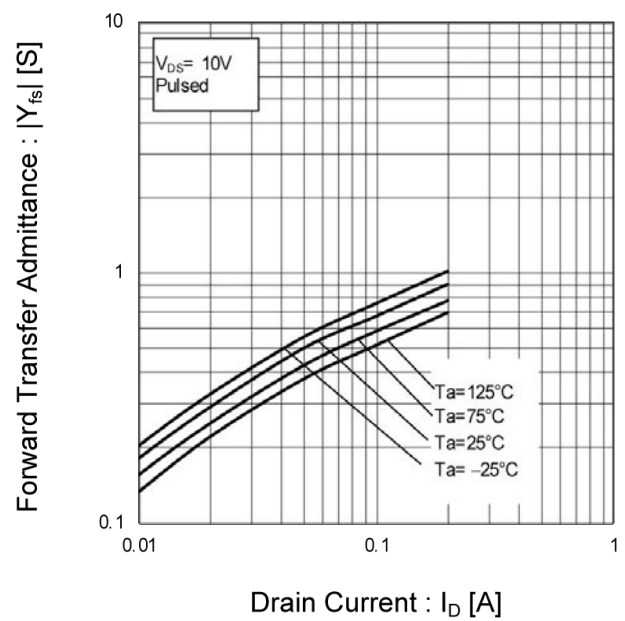
Fig.9 Forward Transfer Admittance vs. Drain Current
