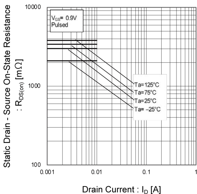
Fig.18 Static Drain - Source On - State Resistance vs. Drain Current (VI)
