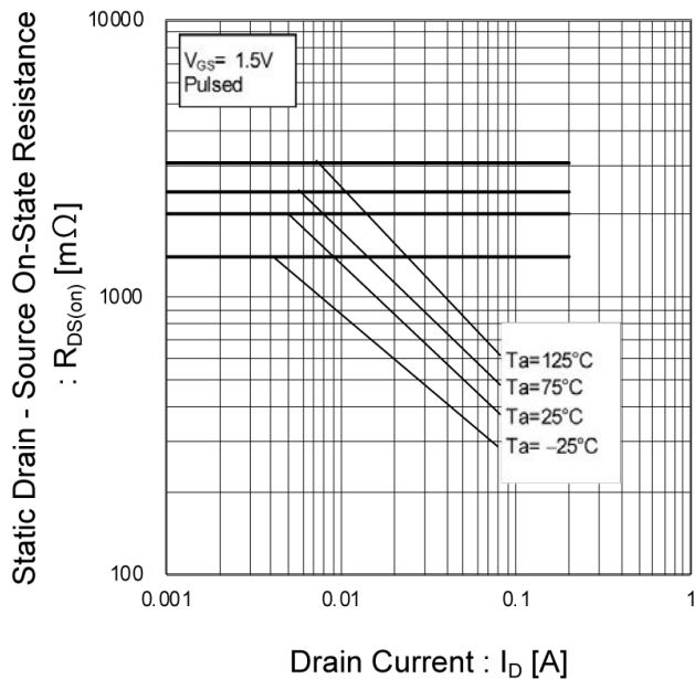
Fig.16 Static Drain - Source On - State Resistance vs. Drain Current (IV)
