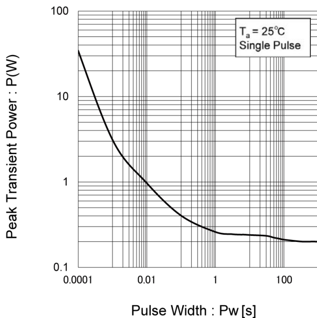
Fig.3 Single Pulse Maximum Power dissipation
