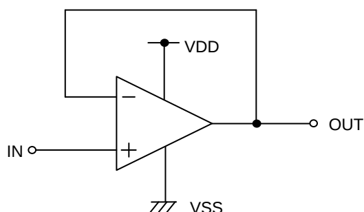
Figure 28. Voltage Follower Circuit
