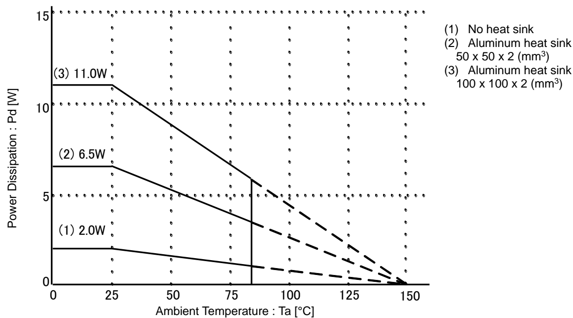
Figure 29. Power Dissipation
