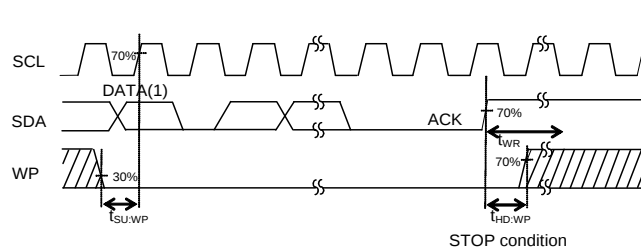
Figure 2-(d). WP Timing at Write Execution
