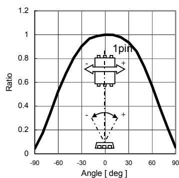
Fig.4 Directional Characteristics 1
