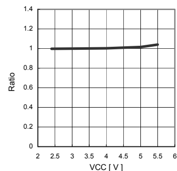
Fig.9 IOUT VCC dependency
