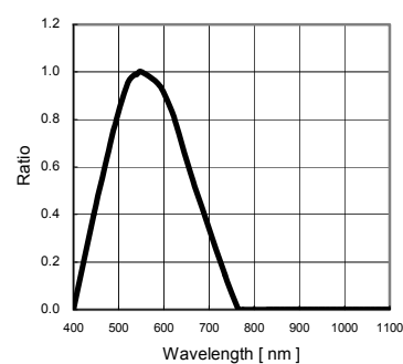
Fig.1 Spectral Response
