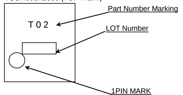
VSON008X2030 (TOP VIEW)
