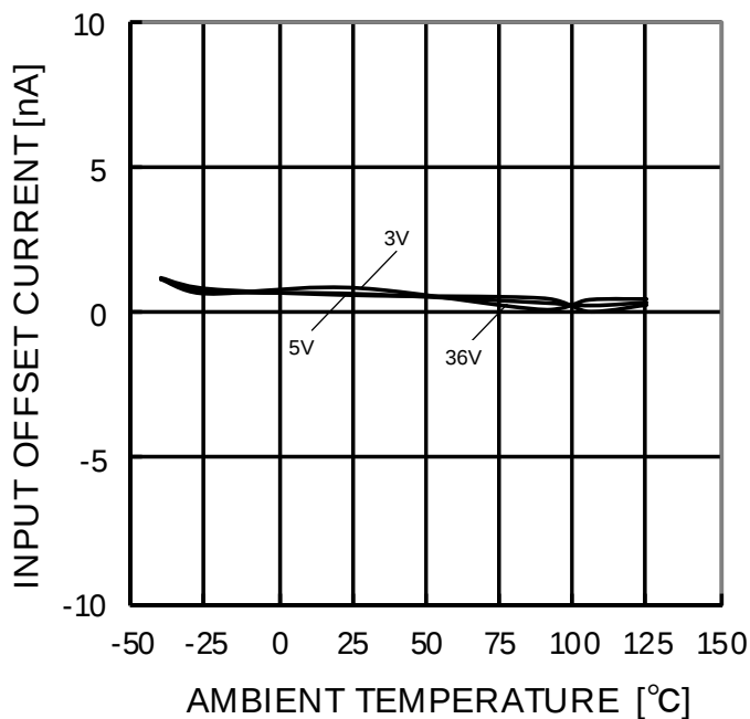
Figure 44. Input Offset Current – Ambient Temperature (Vicm=0V, OUT=1.4V)
