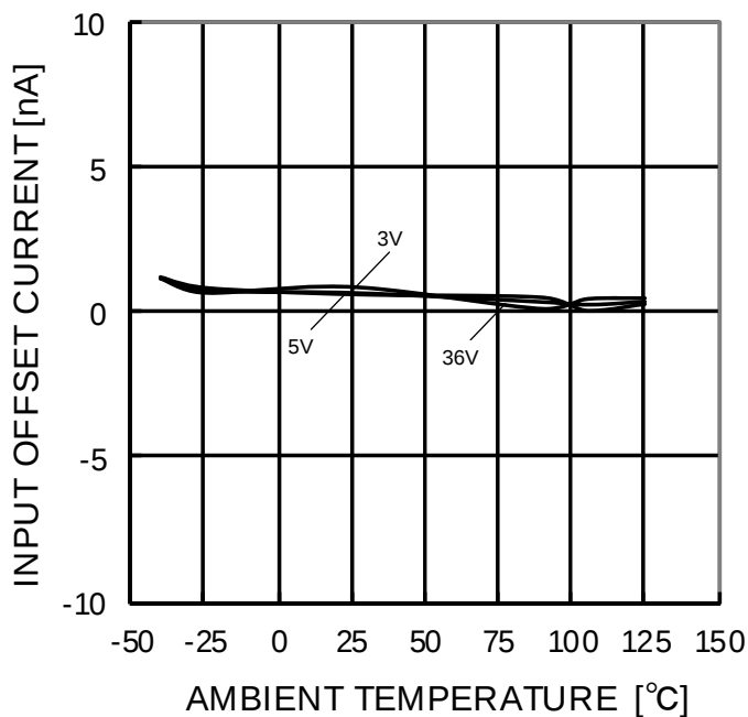
Figure 20. Input Offset Current – Ambient Temperature (Vicm=0V, OUT=1.4V)
