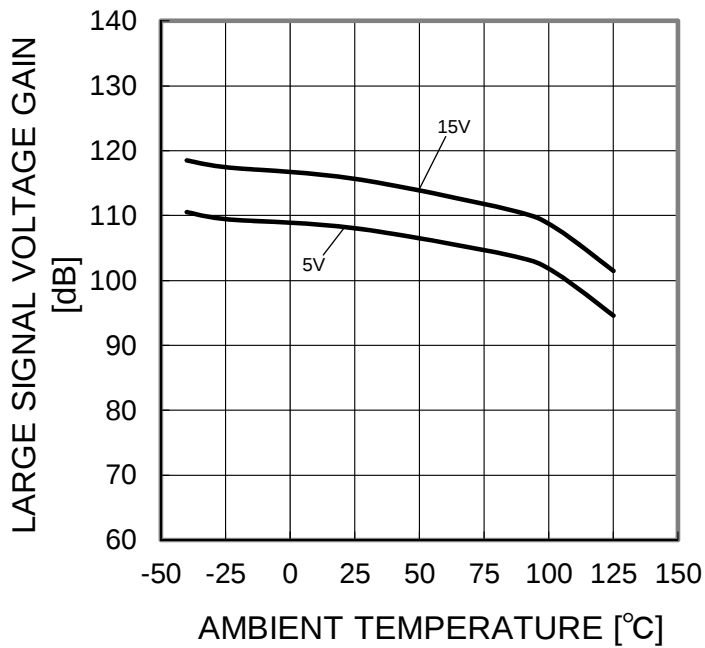
Figure 46. Large Signal Voltage Gain – Ambient Temperature ( R_L=2k\Omega )
