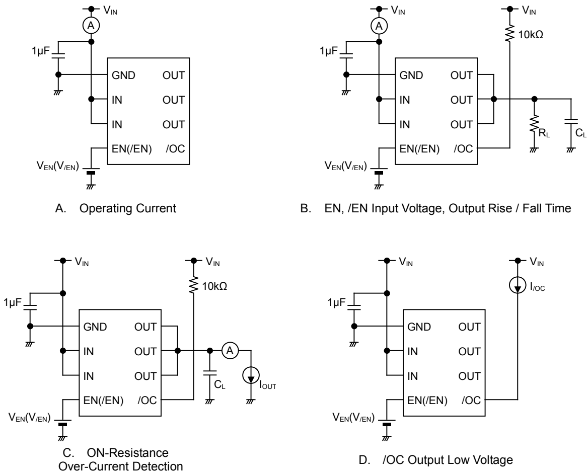
Figure 1. Measurement Circuit
