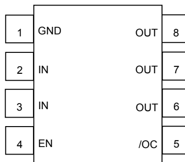
BD82001FVJ (TOP VIEW)
