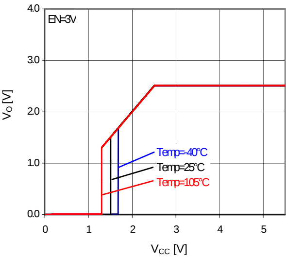
Figure 27. V_{CC} - V_O ( I_O=0mA )
