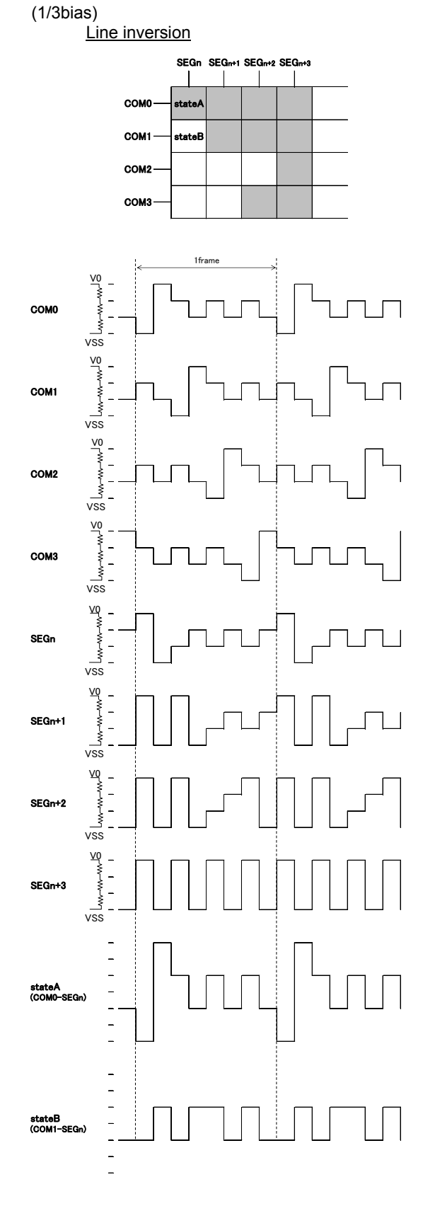
Figure 13. LCD waveform at line inversion (1/3bias)
