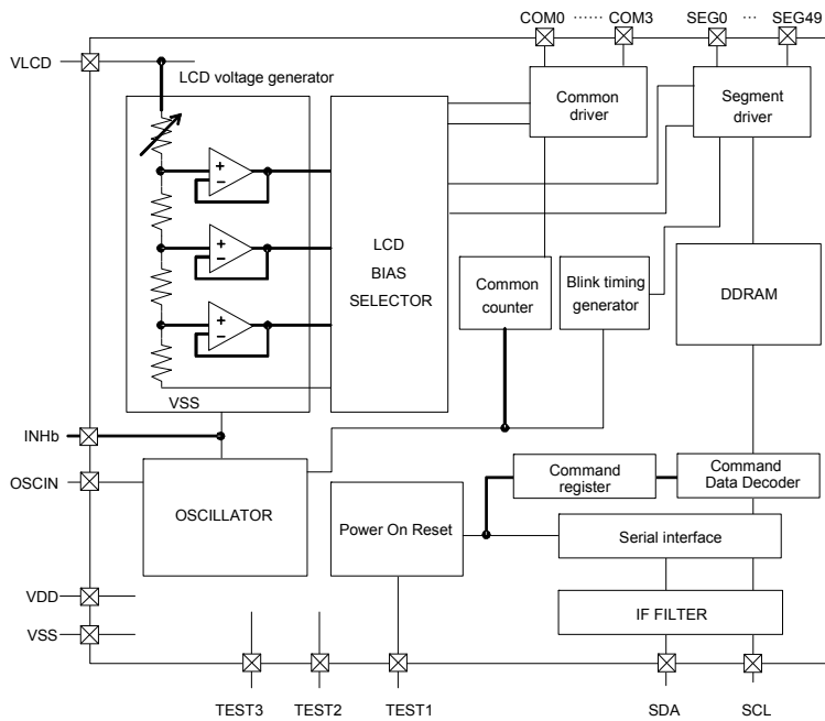
Figure 2. Block Diagram
