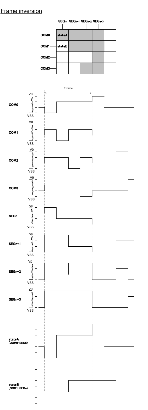
Figure 14. LCD waveform at frame inversion (1/3bias)
