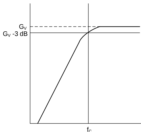
Figure 22. HPF
