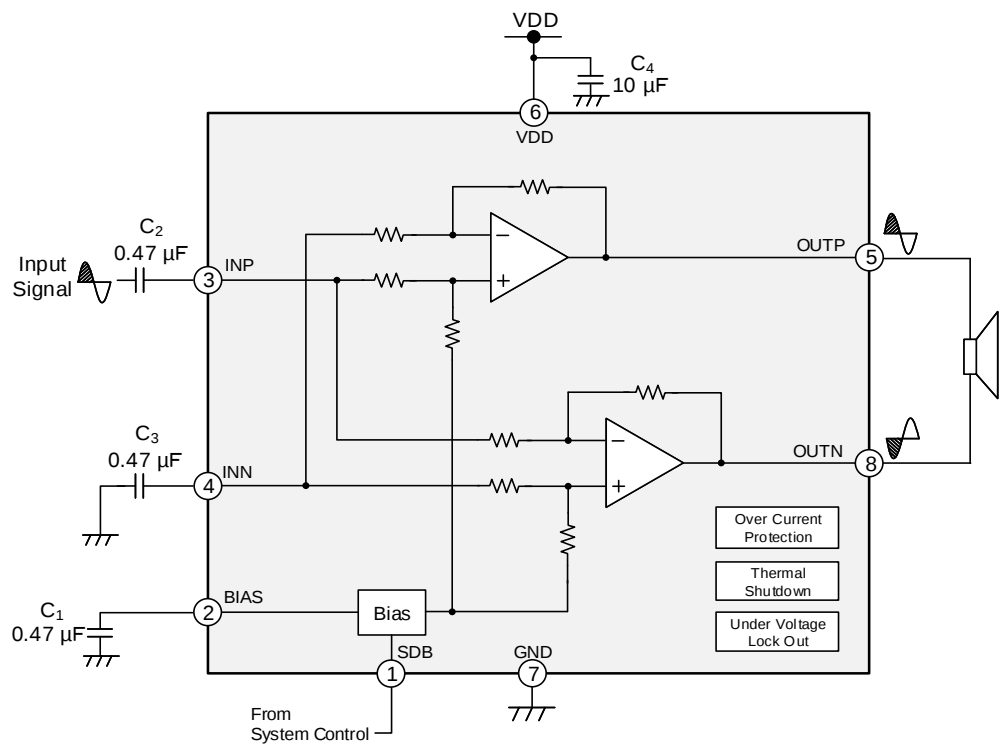
Figure 20. Single-ended Input
