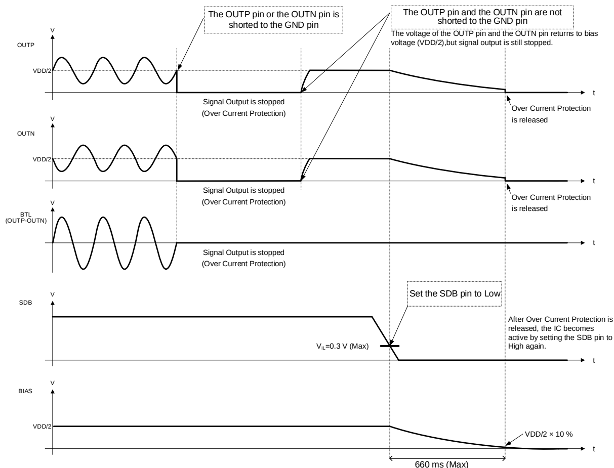
Figure 26. Over Current Protection (Short to the GND pin)
