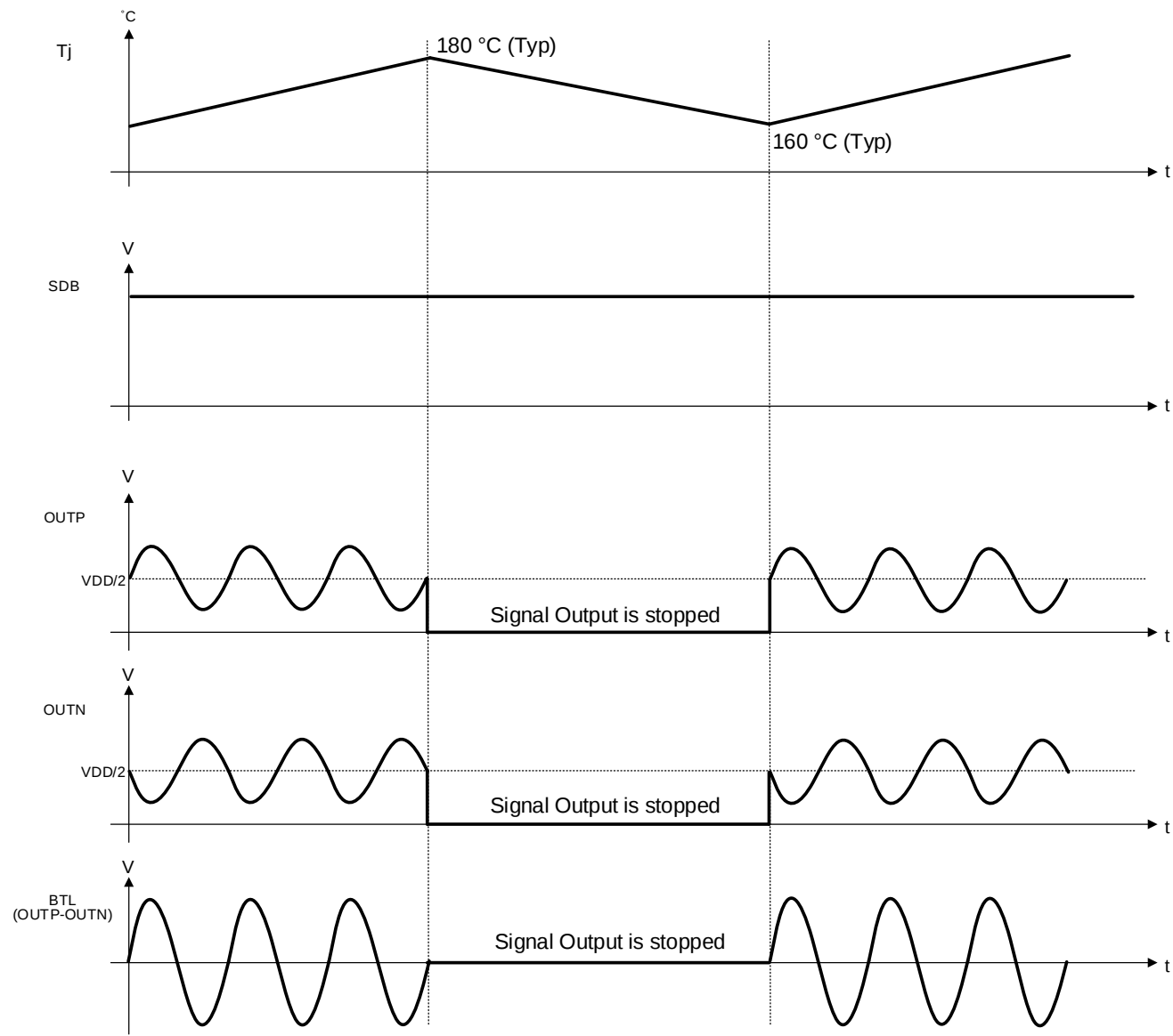
Figure 27. Thermal Shutdown
