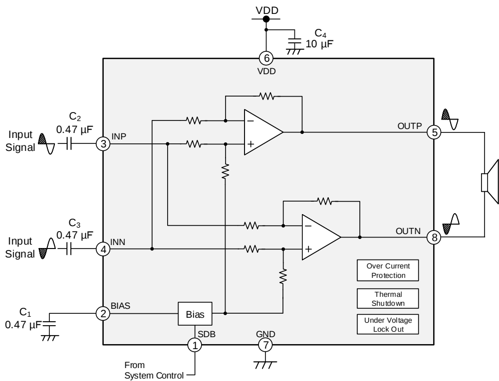
Figure 21. Differential Input
