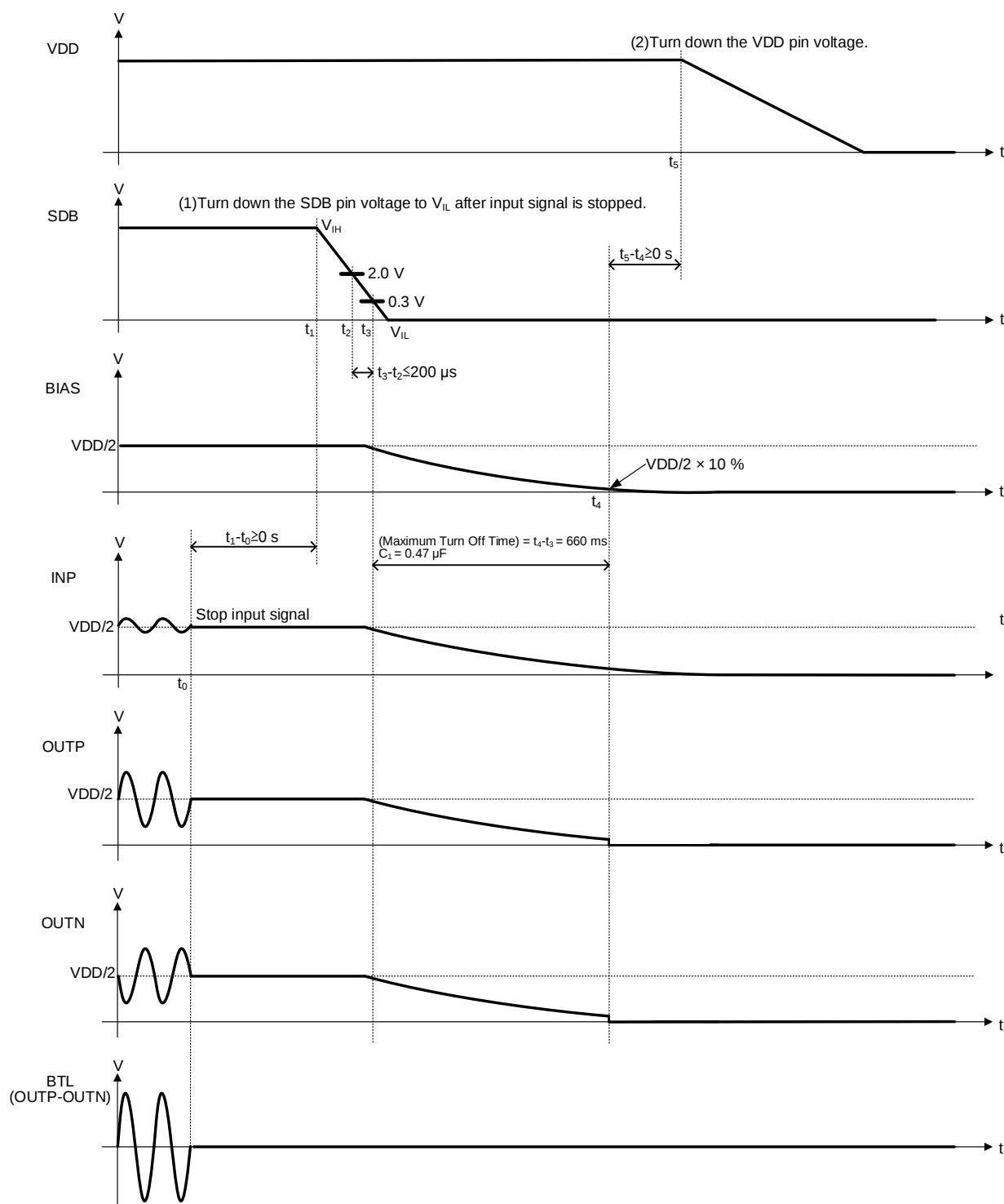
Figure 18. Power Down Sequence
