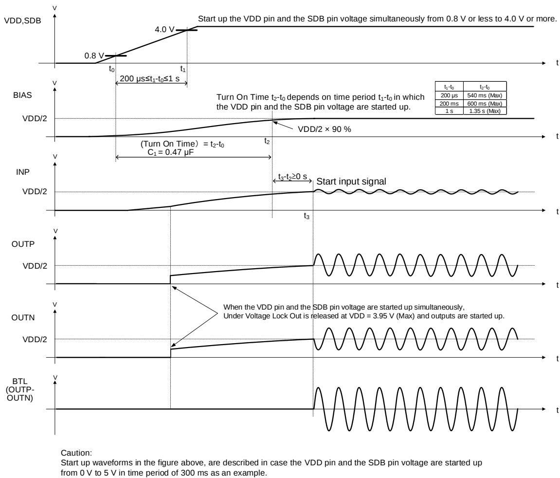
Figure 16. Power On Sequence
