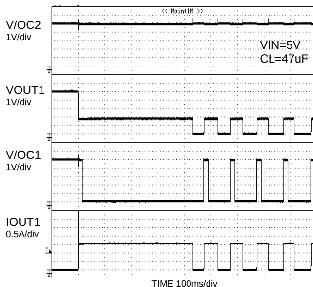
Figure 37. Thermal shutdown response
