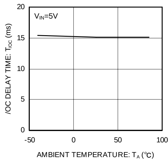
Figure 27. /OC delay time
