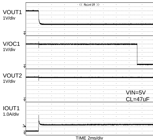
Figure 35. Over-current response 1Ω load connected at enable
