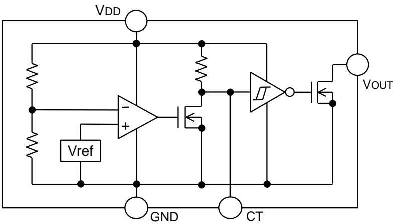
Figure.1 BD52Exxx-M Series
