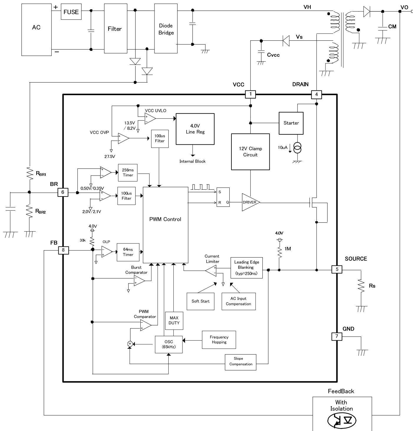
Figure 3. Block Diagram
